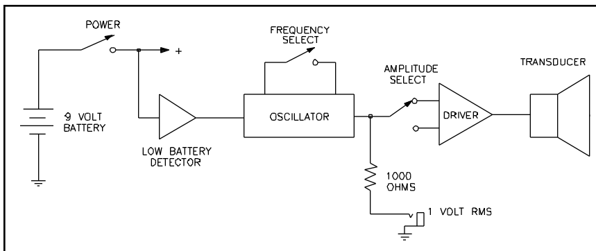
Figure 2. Calibrator Block Diagram
